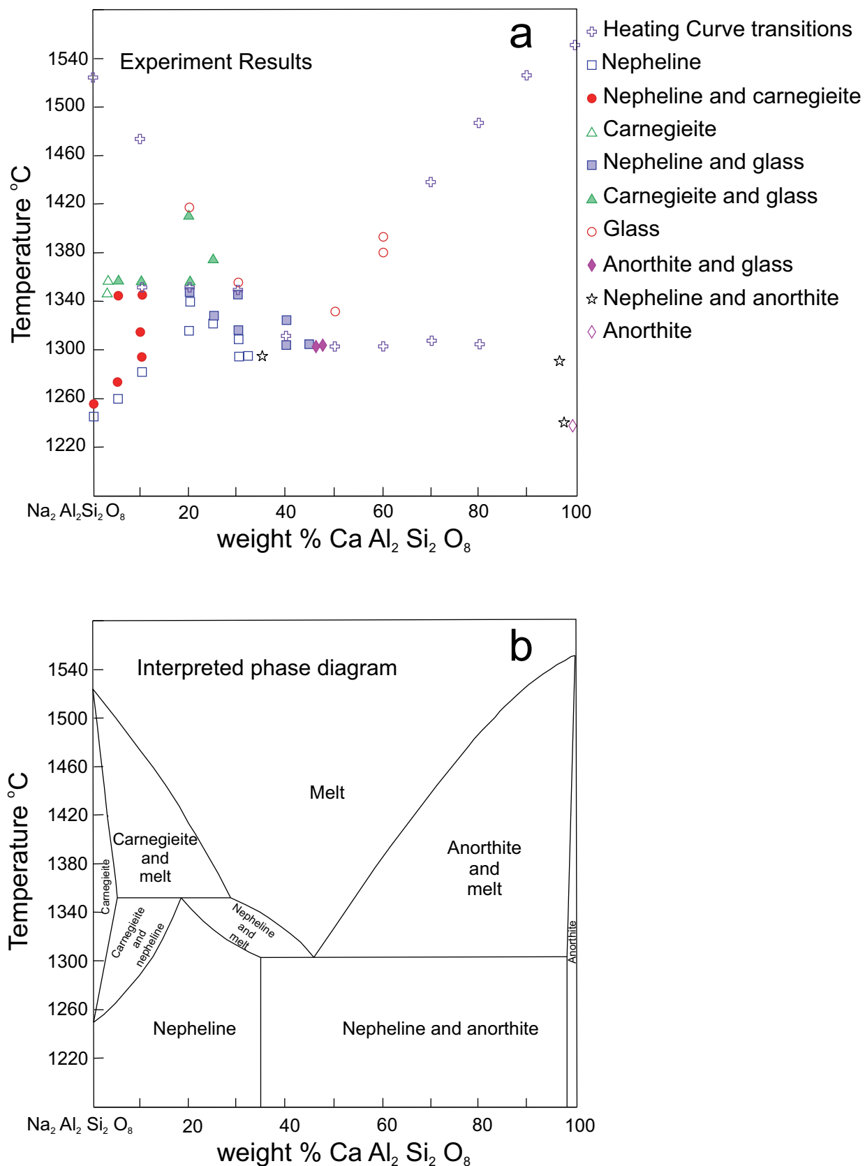
Figure 11. a) The results of Bowen's experiments on the \text{Na}_2\text{Al}_2\text{Si}_2\text{O}_8 – \text{CaAl}_2\text{Si}_2\text{O}_8 system showing the position of transitions defined by the heating curve method and the phases present in long duration quench experiments (Bowen 1912). b) The interpreted phase diagram with no experimental results shown. This is typically the way that phase diagrams are presented to students.
