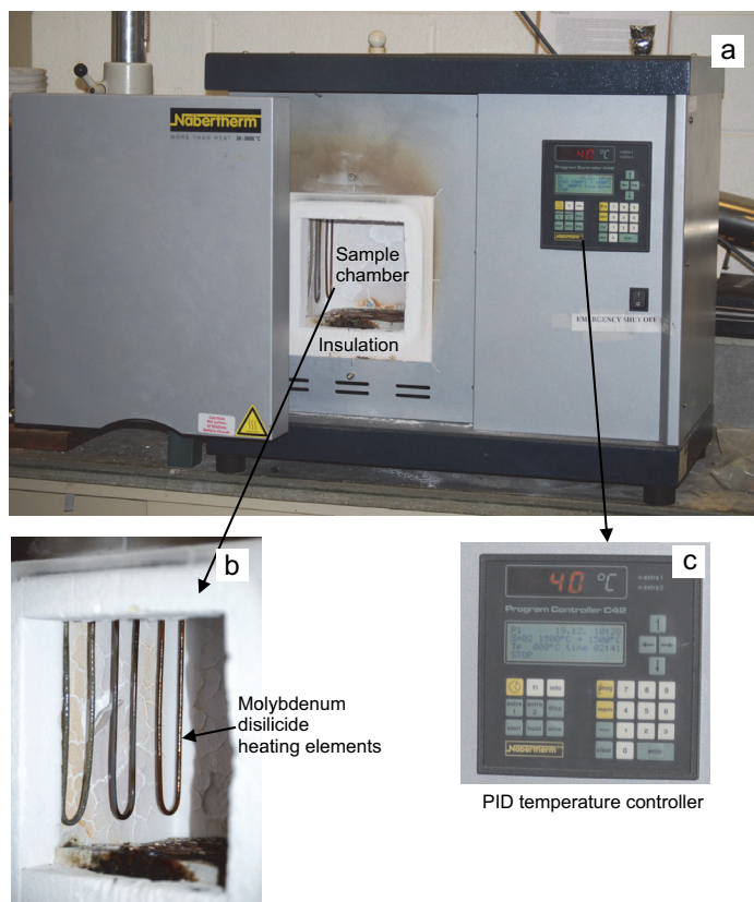
Figure 2. The Nabertherm 1650°C muffle furnace in the experimental petrology laboratory at University of New Brunswick. The sample chamber (a) has a working volume of around 3000 cm 3 . It is heated with U-shaped \text{MoSi}_2 elements (b) and the heating rate, heating duration and final temperature are controlled by the built in digital controller (c).
