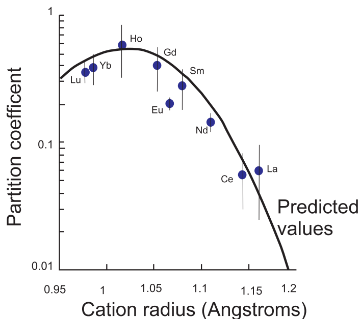
Figure 14. Experimental data of Hart and Dunn (1993) and a model curve calculated using the method of Blundy and Wood (1994). There is close agreement between the measured partitioning values.
