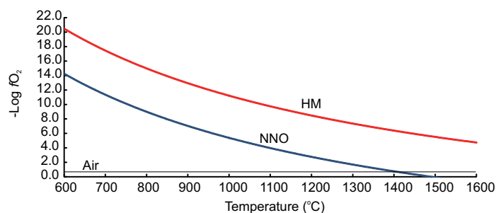
Figure 4. Temperature vs -\log f\text{O}_2 plot showing the position of the relatively reducing Nickel–Nickel oxide (NNO) and oxidizing Hematite–Magnetite (HM) buffer curves. The oxygen fugacity of air is shown for reference.
