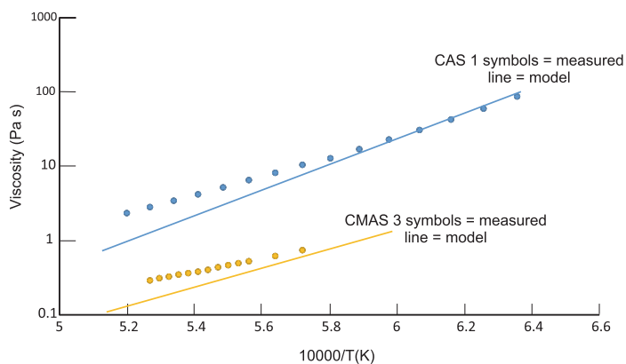
Figure 15. Viscosity measured by rotational viscometry (points) for two synthetic melts in the \text{CaO-Al}_2\text{O}_3\text{-SiO}_2 (CAS) and \text{CaO-MgO-Al}_2\text{O}_3\text{-SiO}_2 (CMAS) systems (Shaw 2006) compared to the viscosity calculated using the model of Giordano and Russell (2007).
